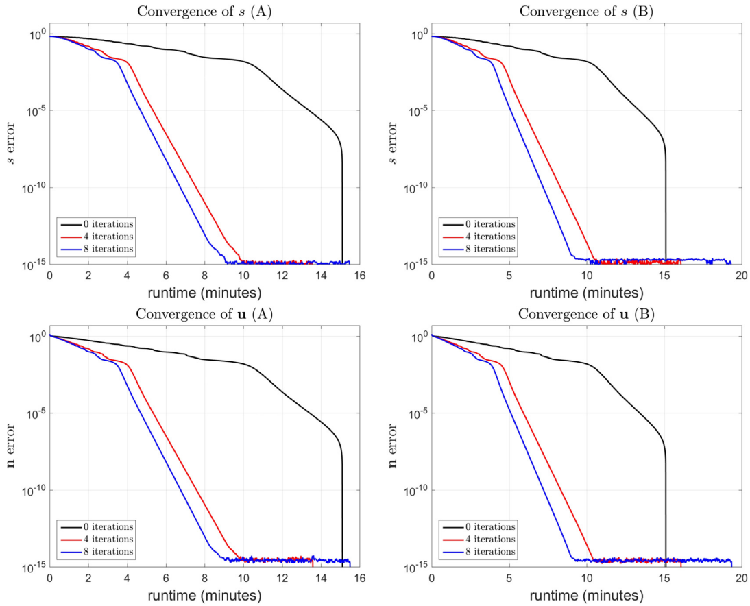
Fig. 3. Ericksen point defect convergence results for s and \mathbf{u} (Section 5.2.1) using the \ell_\infty norm of the error. Plot (A) corresponds to r_1 = 0.2 ; Plot (B) corresponds to r_1 = 0.3 . Number of iterations is for the singular sub-domain \Omega_1^* .
