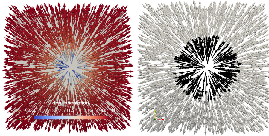
Fig. 2. Point defect at its equilibrium state (Section 5.2.1). Left: director \mathbf{n} is shown colored according to the degree of orientation s ; the minimum value of s is 9.384 \times 10^{-2} . Right: a view of the sub-domain \Omega_1^* in black.
