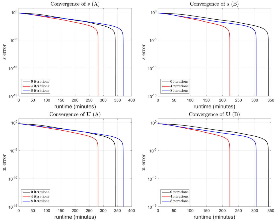
Fig. 7. Uniaxial LdG +1/2 degree defect convergence results for s and \mathbf{U} (Section 5.3.1) using the \ell_\infty norm of the error. Plot (A) corresponds to r_1 = 0.2 ; Plot (B) corresponds to r_1 = 0.3 . Number of iterations is for the singular sub-domain \Omega_1^* .
